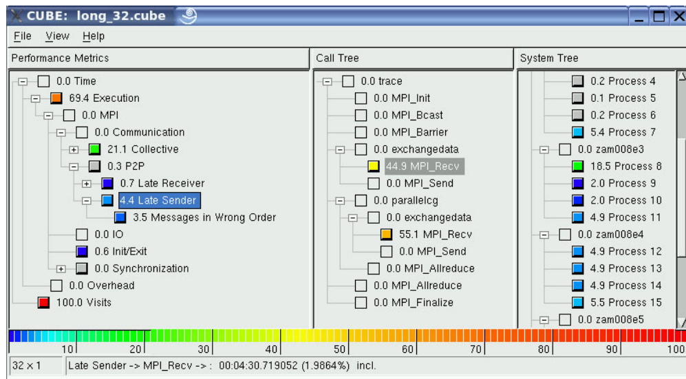
Figure 5. Performance results for MPI application TRACE.
