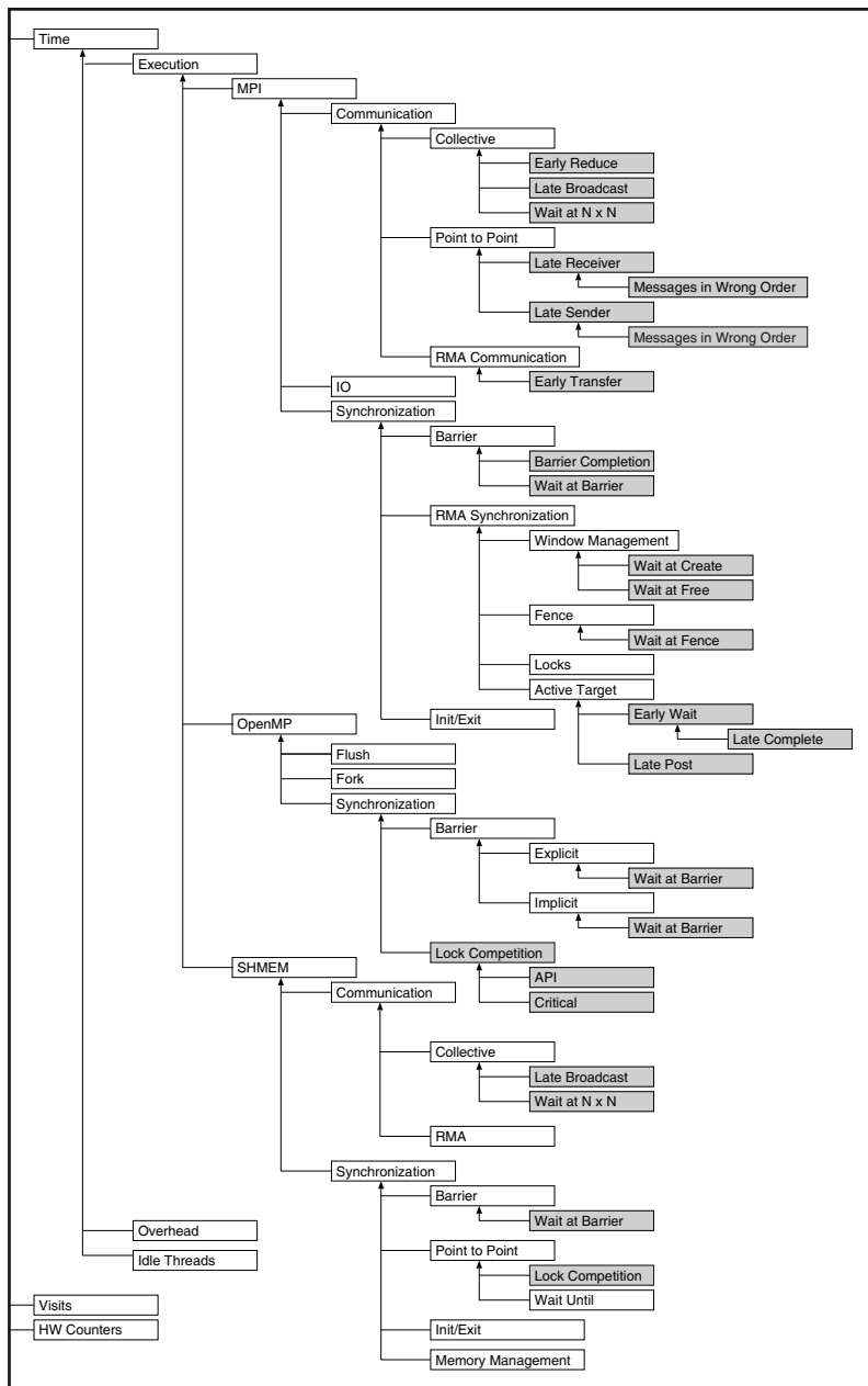
Figure 4. EXPERT pattern hierarchy.
