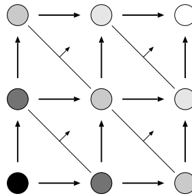
Figure 6. SWEEP3D wavefront propagation.
