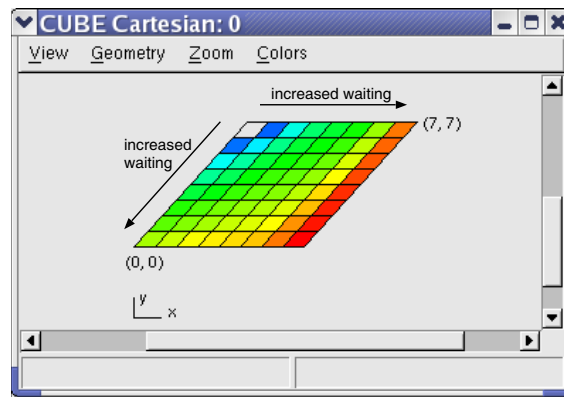
Figure 7. Distribution of late-sender wait states as a result of pipeline refill from the North-West.
