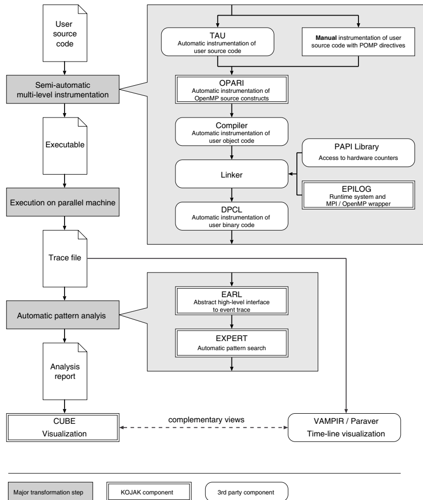
Figure 1. KOJAK architecture.
