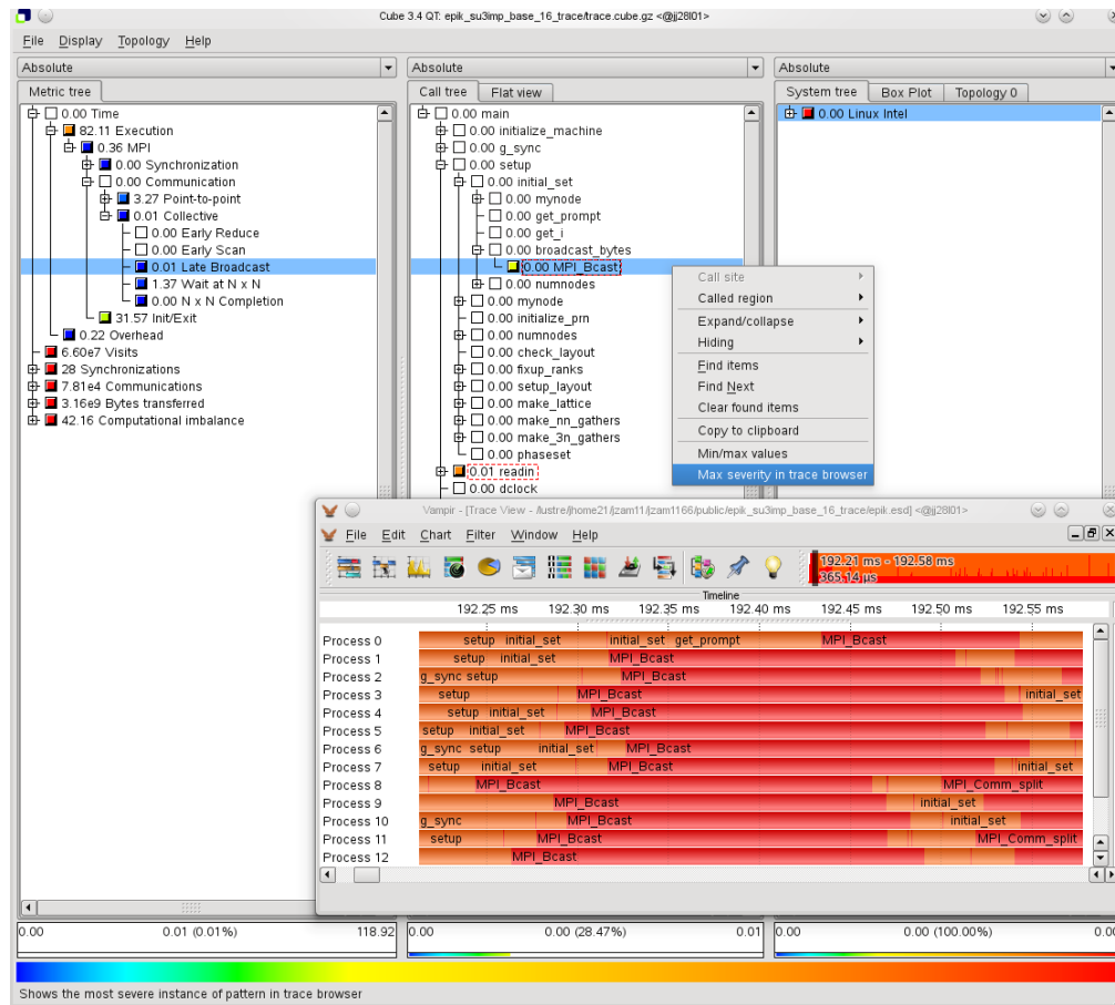
Figure 1.12: Context menu called on a special call path showing the “Max severity in trace browser” menu item which results in the location of the worst Late Broadcast instance shown in the timeline display of Vampir. It can be seen that processes enter the MPI_Bcast operation earlier than the root process leading to a wait state.
